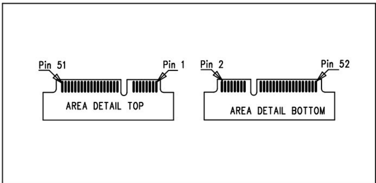
Figure .2-1:Pin Assignment
